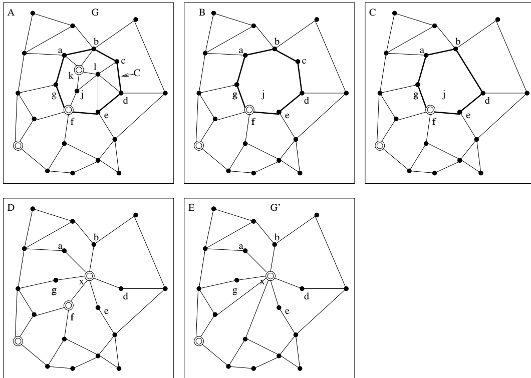
FIGURE 1.11: The Embed operation. Embed finds a cycle C and its subembedding A in an unknown planar embedding of G . Embed removes elements of A that are internal to C , contracting resulting vertices of degree 2 on C , and performs a cycle replacement on C , inserting a new C node x . It then performs contractions to eliminate C -node neighbors of x . The result is the graph G' . By induction on m - n + 1 , a recursive call can be used to find an embedding of G' . Performing a C -node replacement of x gives a planar embedding where C is a face; inverting the foregoing operations inserts the planar embedding of A inside of it.
