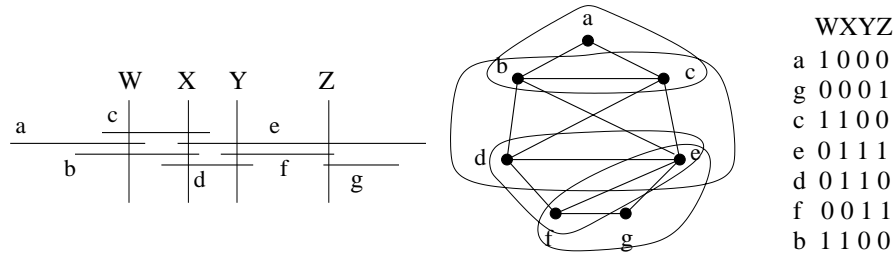
FIGURE 1.3: The clique matrix of a graph has one row for each vertex, one column for each maximal clique, and a 1 in row i column j iff vertex i is contained in clique j . The maximal cliques of an interval graph correspond to points of maximal overlap in an interval representation. Ordering the columns of a clique matrix in the order in which they appear in an interval representation gives a consecutive-ones ordering of the clique matrix.
