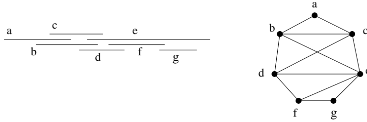
FIGURE 1.2: An interval graph is the intersection graph of a set of intervals on a line. There is one vertex for each of the intervals, and two vertices are adjacent if and only if the corresponding intervals intersect.
