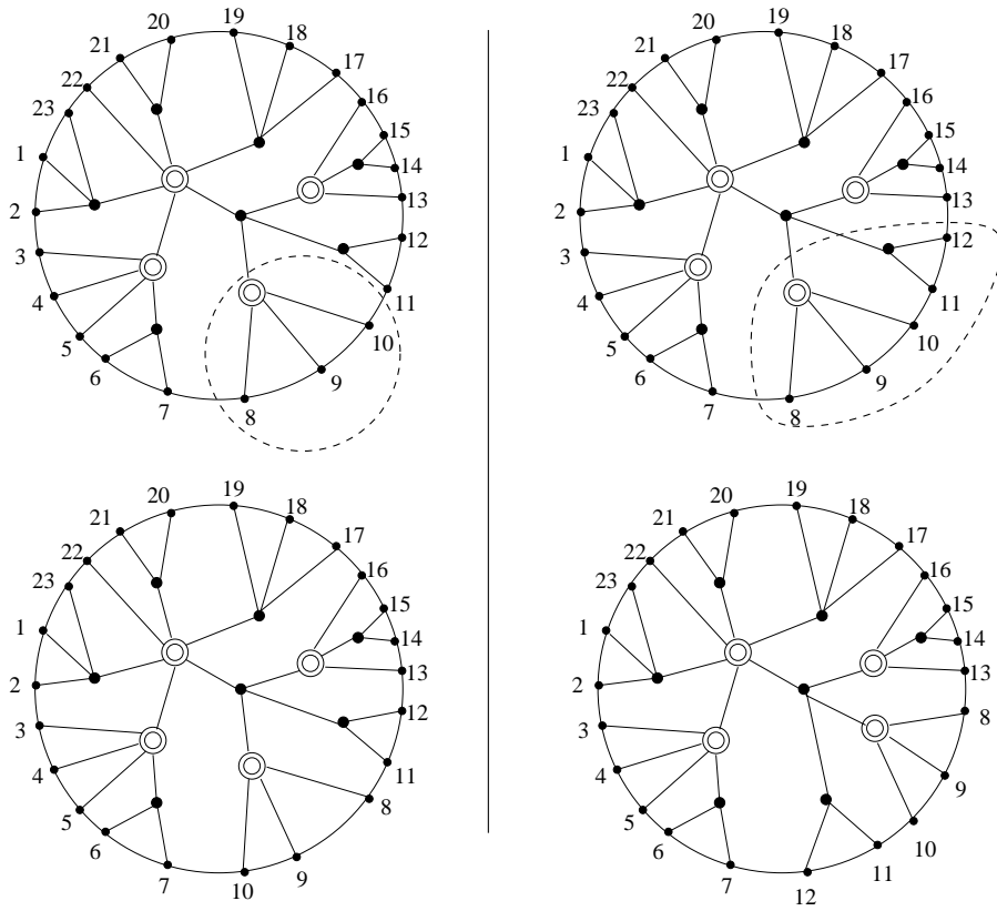
FIGURE 1.5: The PC tree can be viewed as a gadget for generating the circular-ones orderings of the columns. The C nodes are represented by double circles and the P nodes are represented by black dots. The subtree lying at one side of an edge can be flipped over to reverse the order of its leaves. The order of leaves of a consecutive set of subtrees that would result from the removal of a P node can also be reversed. All circular-ones orderings can be obtained by a sequence of such reversals.
