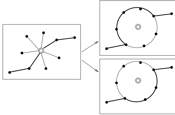
FIGURE 1.13: A C node x of G represents a cycle in H , so a path of G through x represents two possible paths in H .
