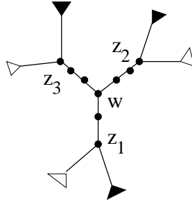
FIGURE 1.14: When the terminal edges of T'_r do not form a path, they form a subtree of T_C with at least three leaves, z_1 , z_2 , and z_3 , each of which is adjacent to a full subtree that has a copy of i and an empty subtree that has a copy of a proper ancestor of i . Let w be the node of the tree from which paths to z_1 , z_2 , and z_3 branch.
