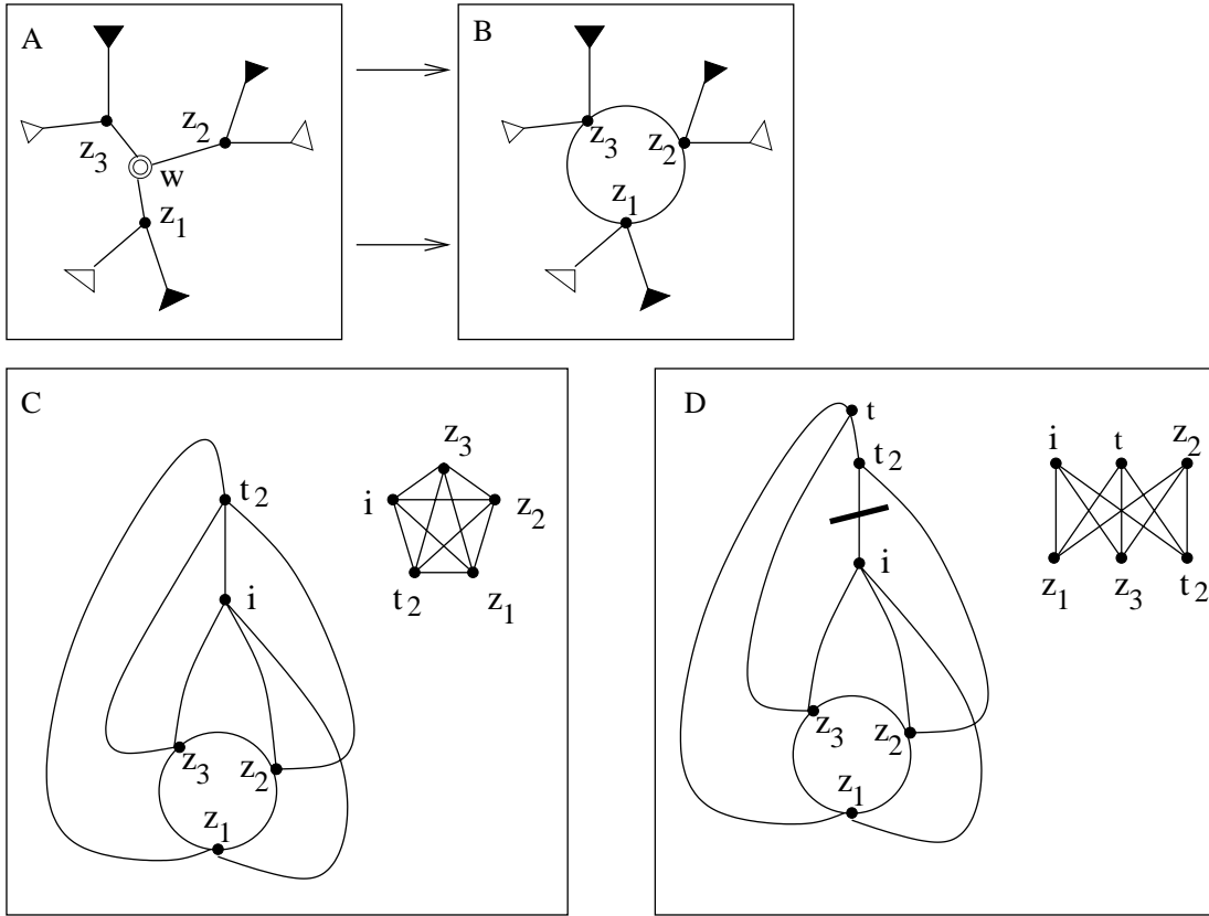
FIGURE 1.17: Each of z_1, z_2 and z_3 is a neighbor of w , which is a C node. Without loss of generality, suppose t_2 is a minimal element of t_1, t_2 , and t_3 . If one of the others, say, t_3 , is equal to t_2 , then the algorithm returns a K_5 . Otherwise, it returns a K_{3,3} .
