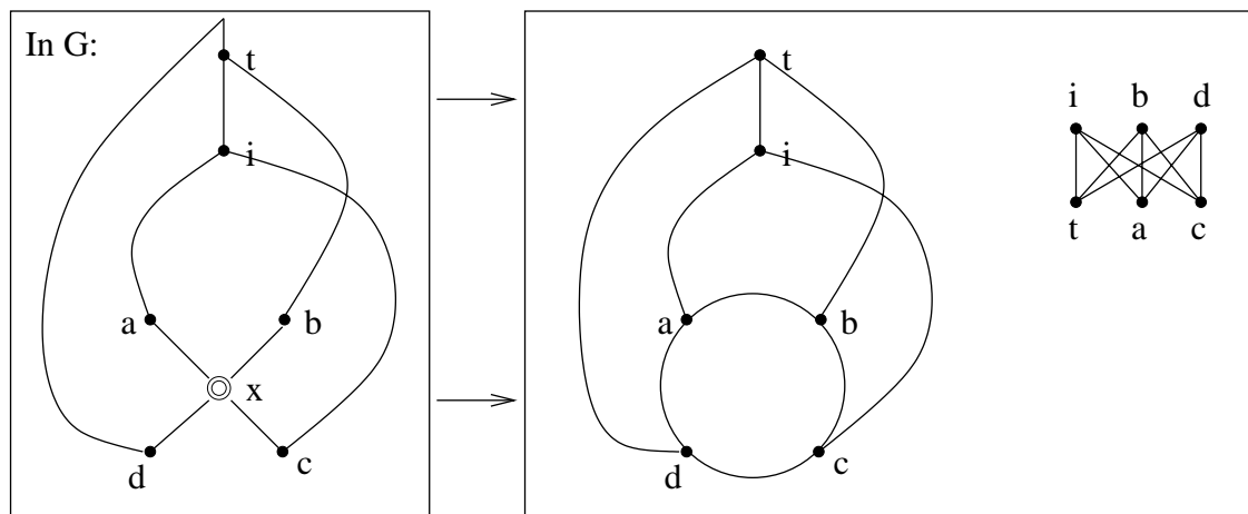
FIGURE 1.18: If a C node x has four neighbors (a, b, c, d) in that order, such that there are disjoint paths from a and c to i and b and d to an ancestor of i , then the cycle that x represents, together with these paths, gives a K_{3,3} .
