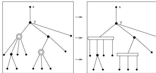
FIGURE 1.6: Assigning a new zero column x to a matrix, computing the PC tree for it, and then picking the PC tree up at x to root it, gives the PQ tree for the matrix, rooted at y , when the C nodes are reinterpreted as Q nodes.
