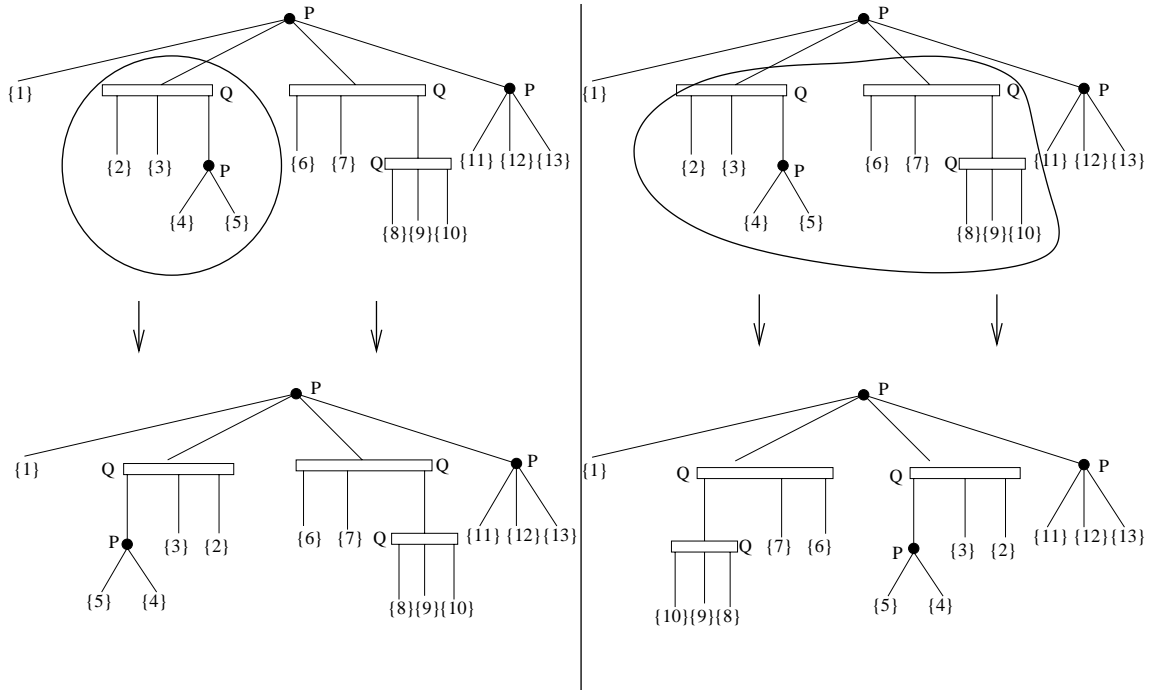
FIGURE 1.4: The leaves of a PQ tree are the columns of a consecutive-ones matrix. The left-to-right order of the leaves gives a consecutive-ones arrangement of the columns. So does the result of reversing the leaf descendants of a node. The order of leaves of a consecutive set of children of a P node can also be reversed to obtain a new consecutive-ones ordering. All consecutive-ones orderings can be obtained by a sequence of these reversals.
