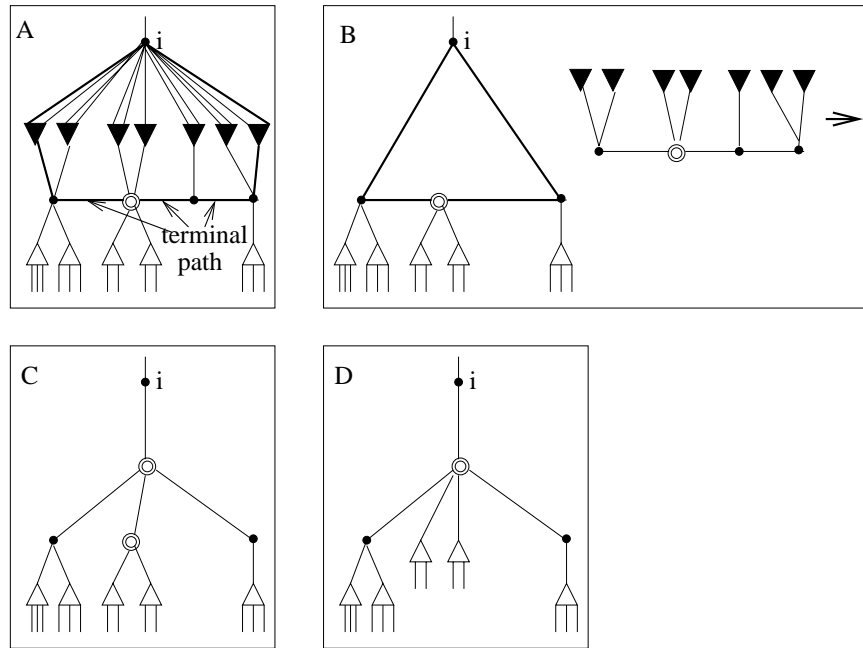
FIGURE 1.12: The induction step of Embed . The cycle C selected by Embed consists of i , the terminal path, and the leftmost and rightmost paths to i from the terminal nodes after full and empty subtrees have been flipped to opposite sides of the terminal path (A). The full nodes and their back edges are trivial to embed inside C , since all of their back edges go to i . The nodes internal to C are to be removed. If they are removed, however, the nodes on the paths from i to the terminal nodes will have degree 2 so they can be contracted out of the cycle. The net effect is to remove all full nodes from G , and leave a cycle consisting of i and the terminal path. This is accomplished by splitting the terminal path, as in the consecutive-ones problem, removing the full side of the split, and inserting an edge from i to each terminal node (B). A cycle replacement is performed on this cycle (C), and, as in the consecutive-ones problem, an order-preserving contraction is performed to remove C -node neighbors of the new C node (D). This yields G' ; performing a recursive call on G' and inverting the steps from A to D on the resulting embedding gives a planar embedding of G .
