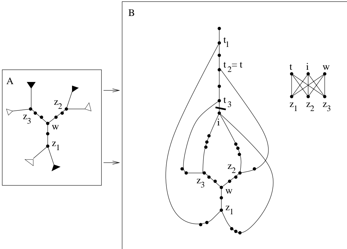
FIGURE 1.15: If w is a P node, S&H gets a K_{3,3} with bipartition \{\{z_1, z_2, z_3\}, \{w, i, t\}\} . This K_{3,3} is the contraction of a K_{3,3} of the original input graph H .
