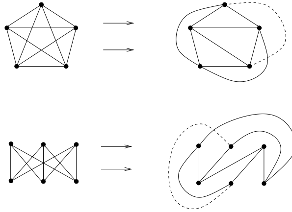
FIGURE 1.1: Two non-planar graphs. The first is the K_5 , the complete graph on five vertices, and the second is the K_{3,3} , the complete bipartite class on two sets of three vertices each. Any attempt to embed them in the plane fails when a final edge cannot be inserted without crossing the boundary between two faces.
