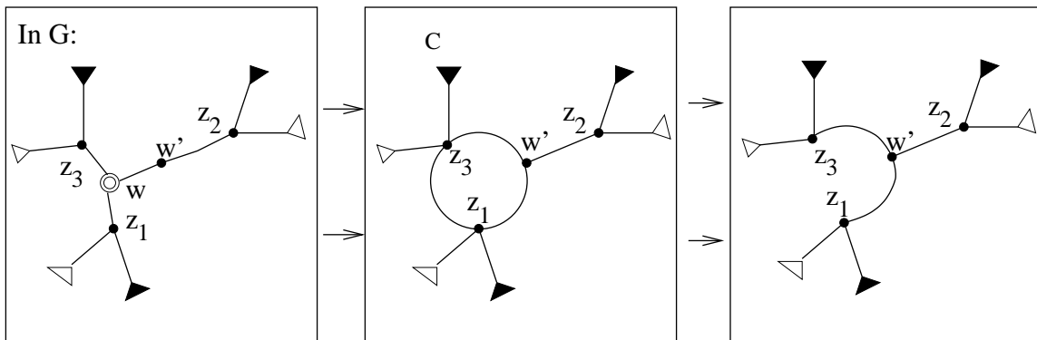
FIGURE 1.16: If w is a C node but at least one of z_1, z_2, and z_3 is a non-neighbor of w , the case can be reduced to that of Figure 1.15 by selecting a neighbor w' to serve in the role of w .
