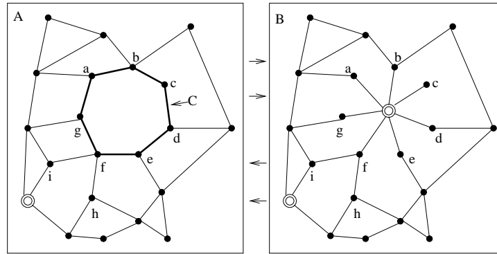
FIGURE 1.10: A cycle replacement consists of selecting a cycle in a graph, adding a new C node whose neighbors ordering gives the ordering of nodes on the cycle, and deleting the edges of the cycle. As we illustrate in parts C and D of Figure 1.11, below, it is applied to a graph that arises partway into the induction step. It's inverse operation is a C -node replacement.
