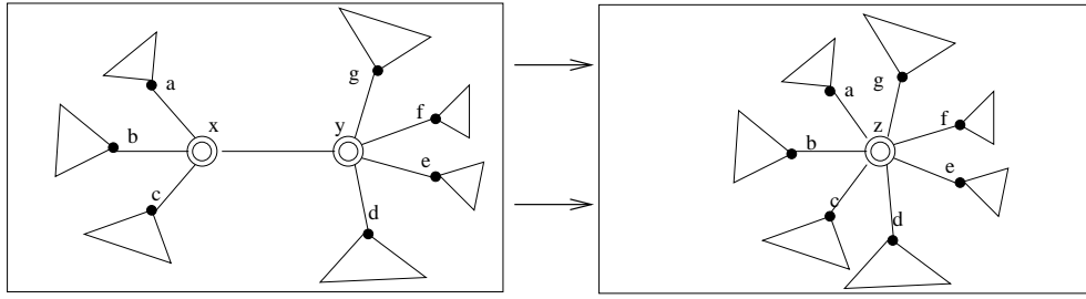
FIGURE 1.9: An order-preserving contraction of an edge xy . The neighbors of x and y are cyclically ordered. The edge is removed and x and y are identified, so that the cyclic order of neighbors of x and y about the edge is preserved.
