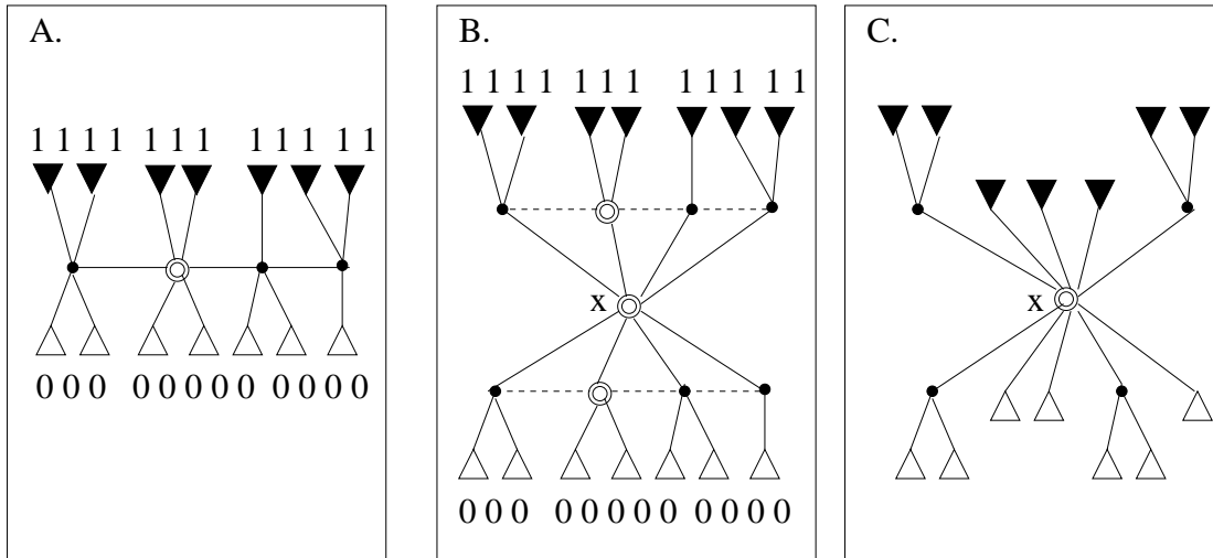
FIGURE 1.8: To update the PC tree when a new row is added to the matrix, flip the C nodes and order the P nodes on the terminal path so that the edges that go to trees whose leaves are zeros in the row lie on one side (white) and those that go to trees whose leaves are ones in the row lie on the other side (black). This is always possible if the new matrix has the circular-ones property (Figure A). Then divide each node on the terminal path into two parts, one that is adjacent to the black trees and one that is adjacent to the white trees (Figure B). Replace the edges of these two paths with a new C node, x , whose cyclic order reflects the order of nodes these two paths. Finally, contract each edge from x to a C-node neighbor, and contract each internal node of degree two (Figure C).
