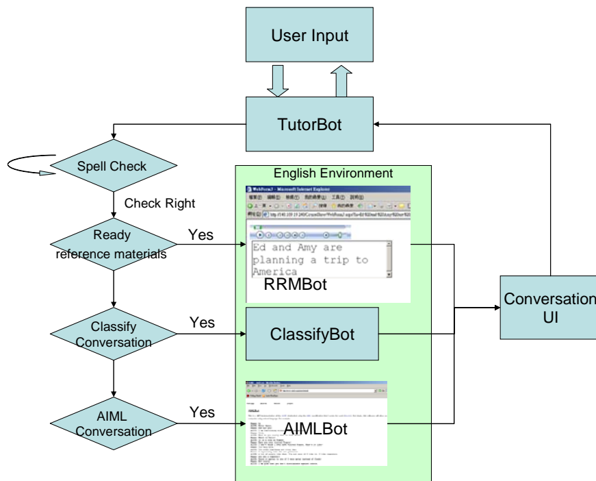
Fig. 3. Conversation flow chart
