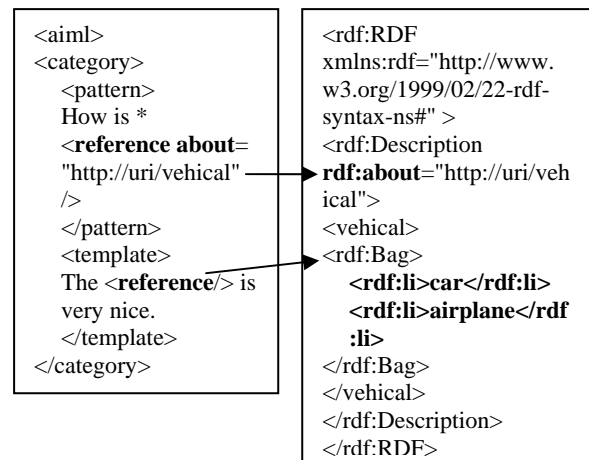
Figure 5 Example of Term-expansion
