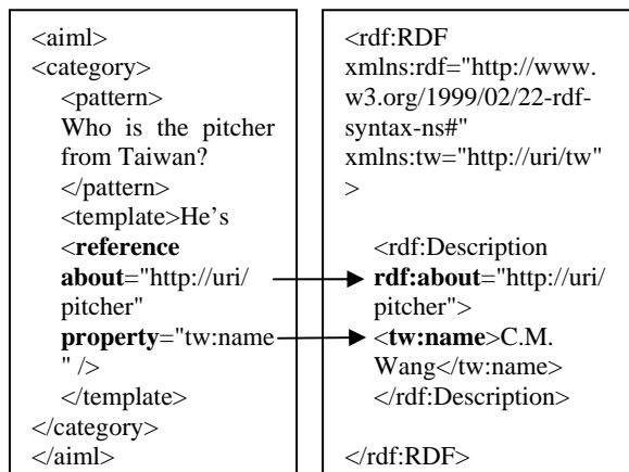
Figure 2 Example of Template-side Reference
