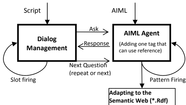
Figure 6 Experiment Architecture
