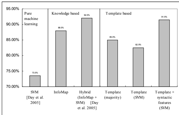
Fig. 1. Fine-grained accuracy of the proposed approaches and a knowledge-based approach.
