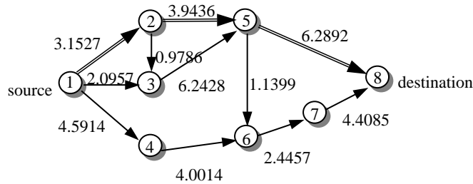
Fig. 7. The fuzzy network G = (V, E) with \{c_{ij}^\circ \mid i, j \in E\} .
