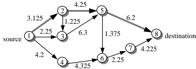
Fig. 5. The fuzzy network G = (V, E) with \{c_{ij}^* | i, j \in E\} .
