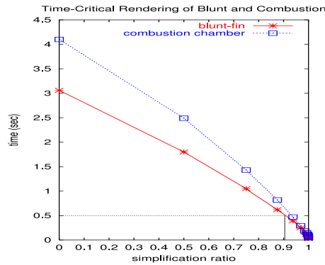
Fig. 5. Time-critical rendering of the Blunt-fin and Combustion Chamber datasets for different simplification ratios. Image resolution is set at 128 \times 128 .
