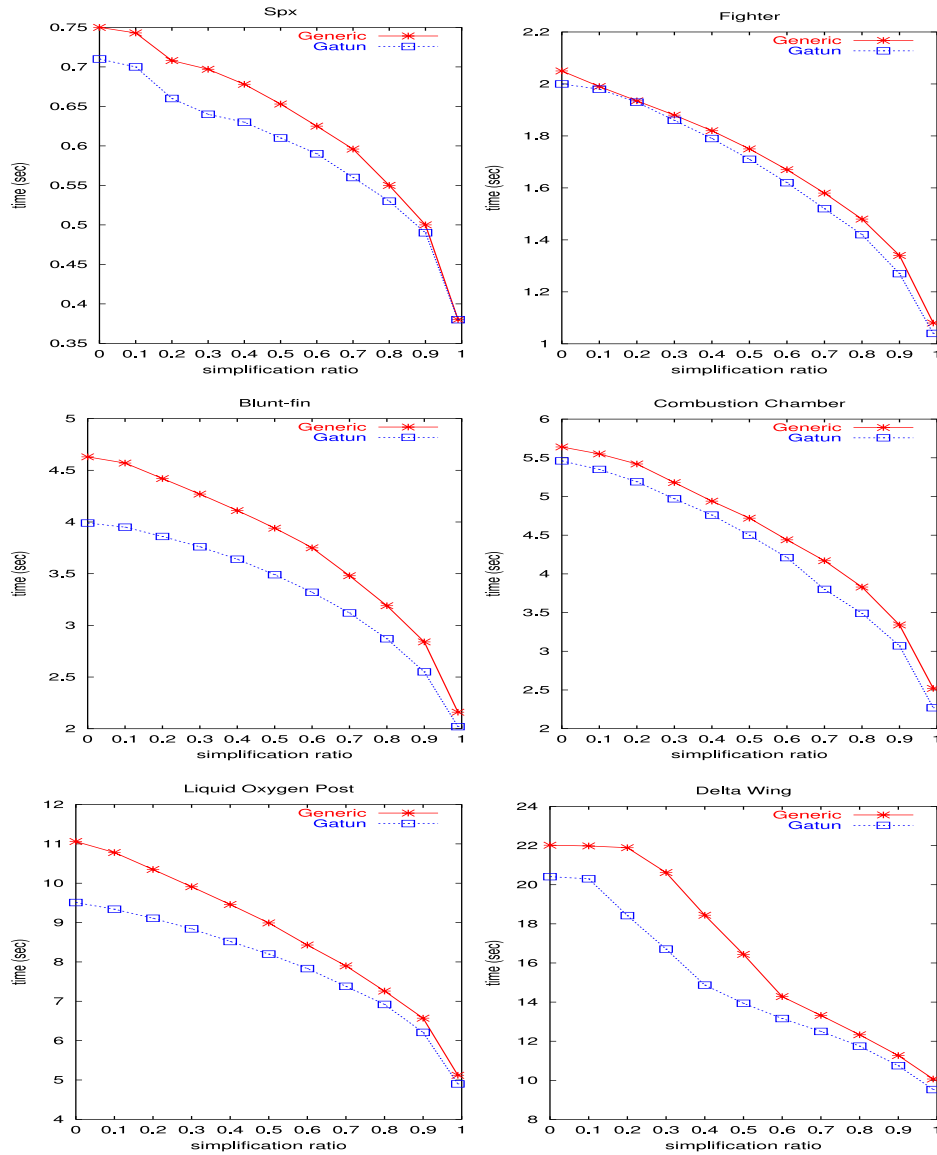
Fig. 4. Comparisons between the generic renderer (the baseline) and Gatun for different simplification ratios. There is only one version of the input dataset stored on the disk. Image resolution is set at 256 \times 256 .
