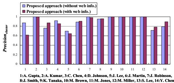
Fig. 3. The clustering precision of each dataset
