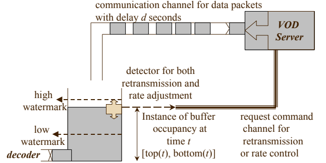
Figure 4. Error control model for the True VOD system
