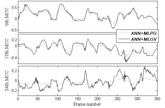
Fig. 2: Example trajectories of MCC features converted by the proposed ANN-based VCs.
