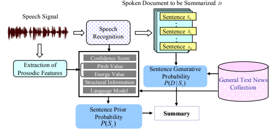
Figure 1: A schematic depiction of extractive spoken document summarization using the probabilistic generative framework.
