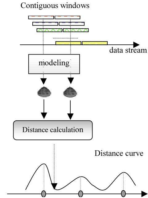
Figure 1. The procedures of metric-based segmentation
