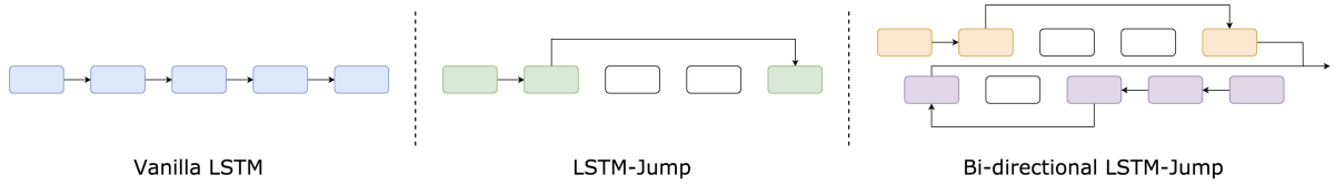
Figure 2: Baseline architectures. Left: Vanilla LSTM: reads entire text sequentially. Middle: LSTM-Jump: skims to neglect some words. Right: Bi-direction LSTM-Jump: skims in two directions, concatenates two latest hidden states.
