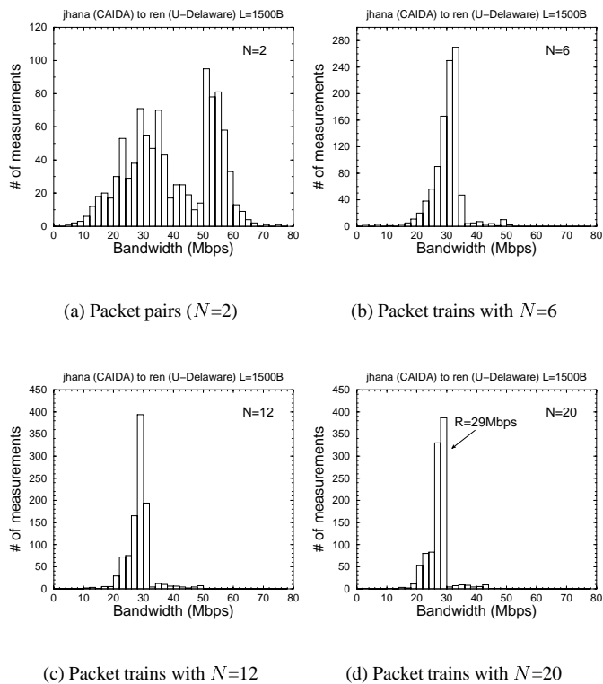
Fig. 8. The effect of the packet train length (measurements).
